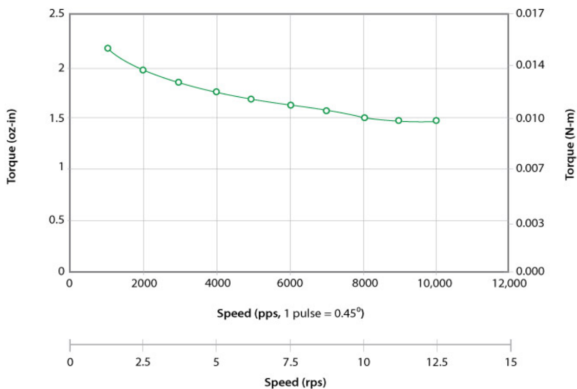
4109Z-51 24VDC, 0.5 Amps/Phase, Bipolar, 1/2 Stepping
